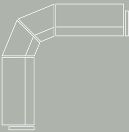
90° External & Straight Units with Arms Footprint: W2310 x D2310 (min)
